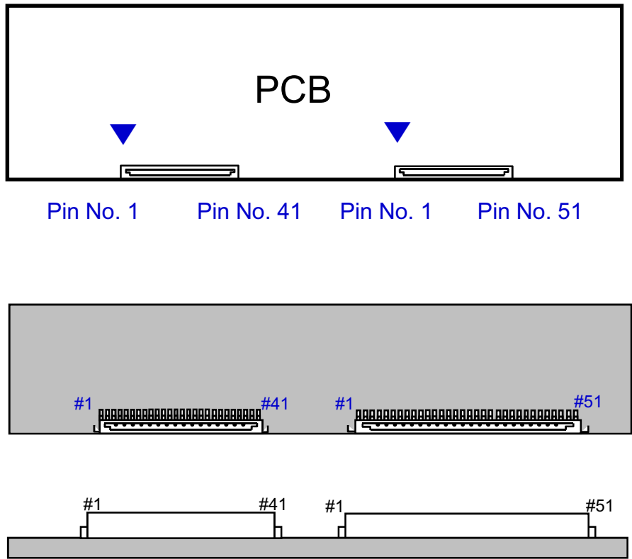
Fig. Connector diagram
